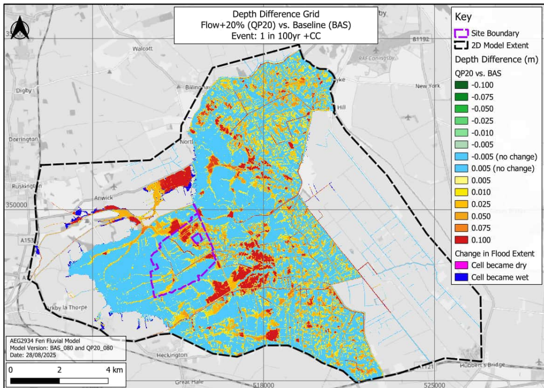
Figure 24: Depth Difference Grid - 20% increase flows vs Baseline (unfiltered). Event: 1 in 100-year + CC. (Base map from OpenStreetMap and OpenStreetMap Foundation (CC-BY-SA). © and contributors)
