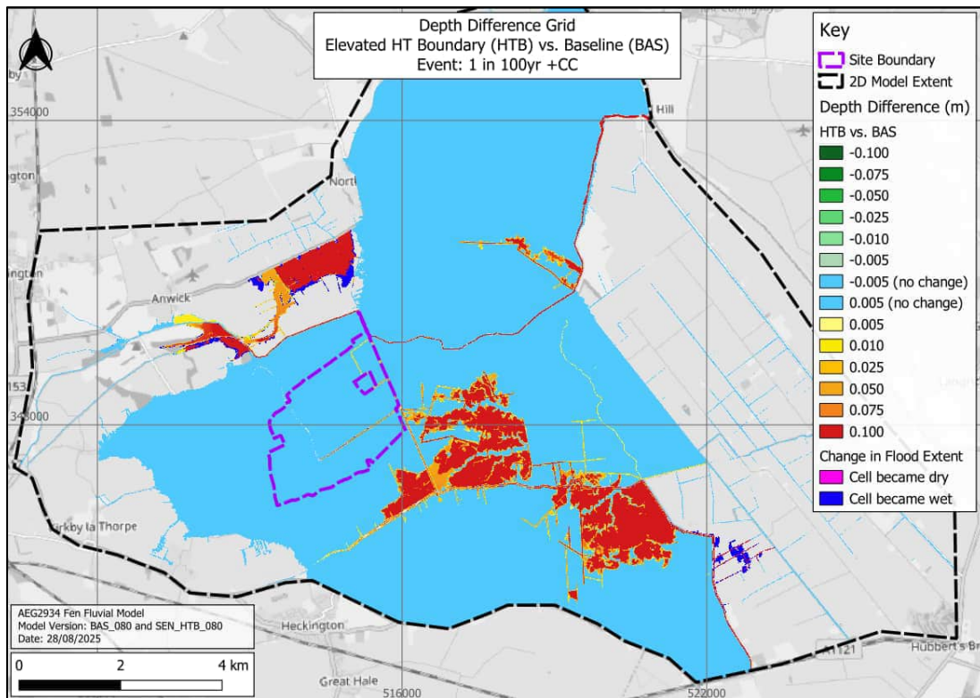
Figure 36: Depth Difference Grid - Elevated HT downstream boundary vs Baseline (unfiltered). Event: 1 in 100-year + CC. (Base map from OpenStreetMap and OpenStreetMap Foundation (CC-BY-SA). © [redacted] and contributors)
