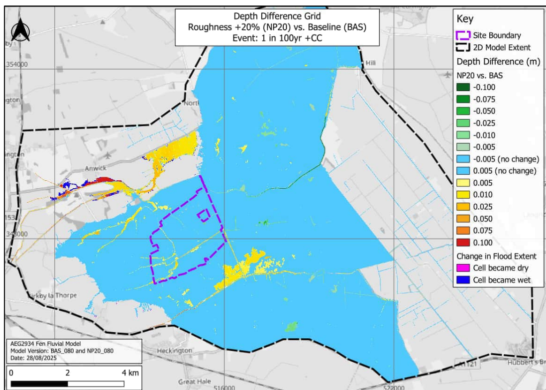
Figure 26: Depth Difference Grid - 20% Increase Manning's n (1D & 2D) vs Baseline (unfiltered). Event: 1 in 100-year + CC. (Base map from OpenStreetMap and OpenStreetMap Foundation (CC-BY-SA). © and contributors)
