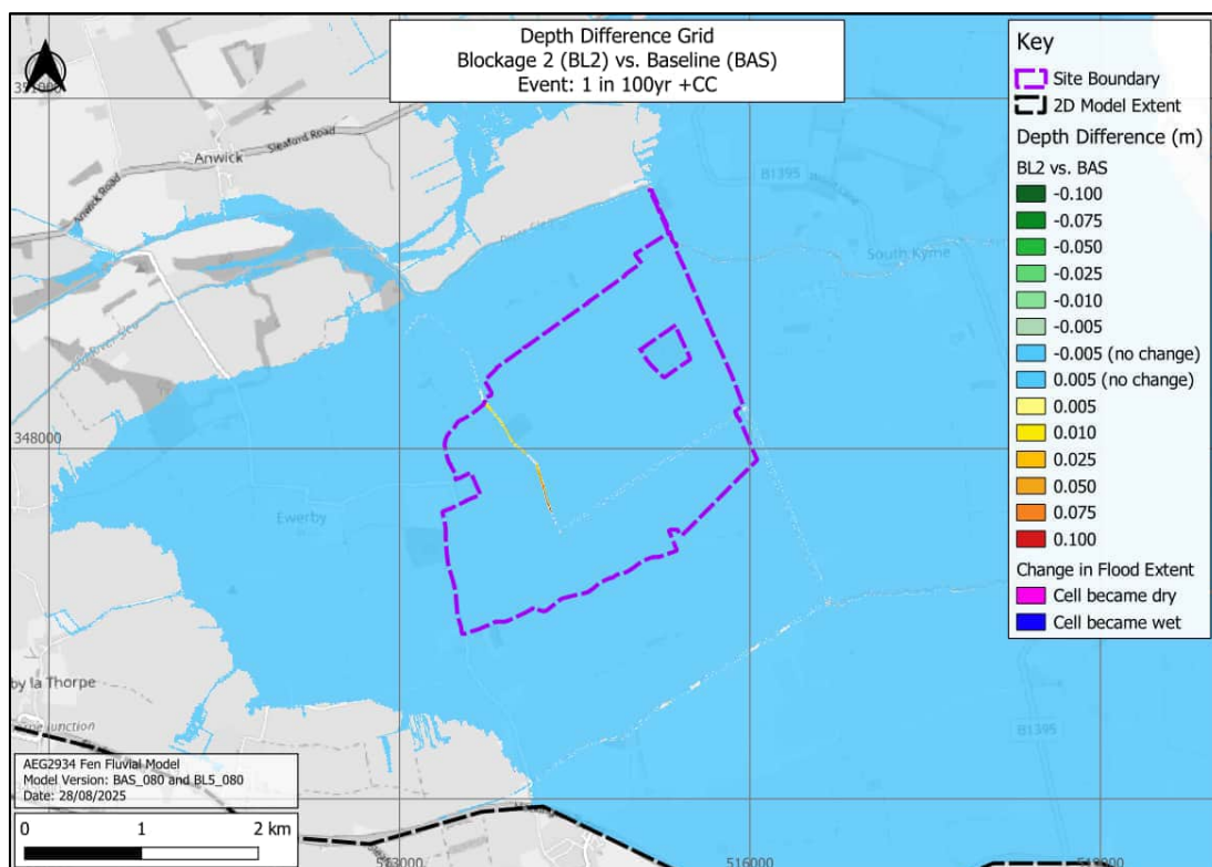
Figure 34: Depth Difference Grid - Blockage 2 (Black Sluice, 100%) vs Baseline (unfiltered). Event: 1 in 100-year + CC. (Base map from OpenStreetMap and OpenStreetMap Foundation (CC-BY-SA). © [redacted] and contributors)
