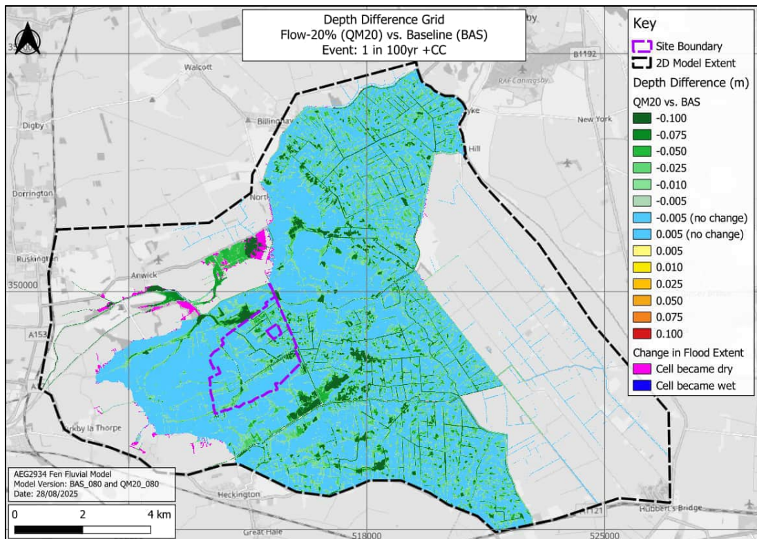
Figure 25: Depth Difference Grid - 20% decrease flows vs Baseline (unfiltered). Event: 1 in 100-year + CC. (Base map from OpenStreetMap and OpenStreetMap Foundation (CC-BY-SA). © and contributors)
