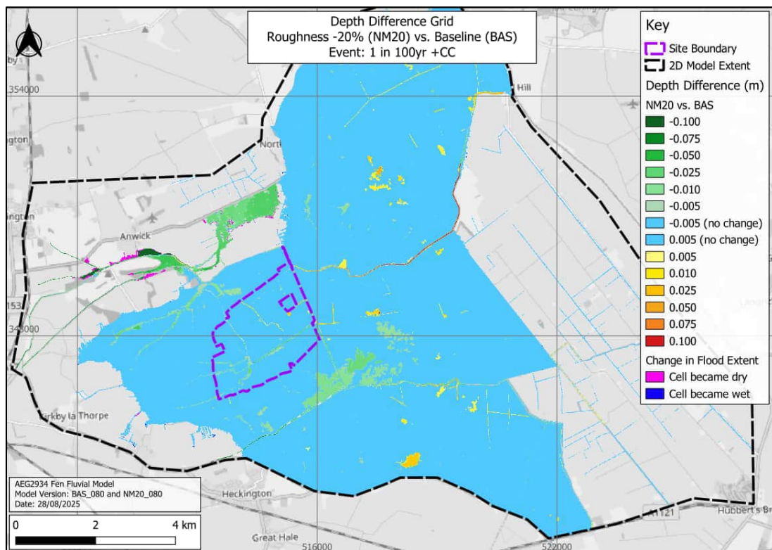
Figure 27: Depth Difference Grid - 20% Decrease Manning's n (1D & 2D) vs Baseline (unfiltered). Event: 1 in 100-year + CC. (Base map from OpenStreetMap and OpenStreetMap Foundation (CC-BY-SA). © and contributors)
