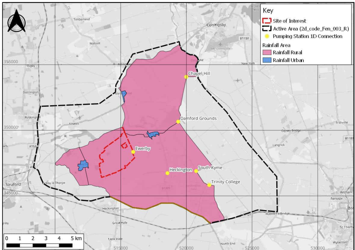
Figure 14: 2D Boundary Locations (Base map from OpenStreetMap and OpenStreetMap Foundation (CC-BY-SA). © https://www.openstreetmap.org and contributors)
