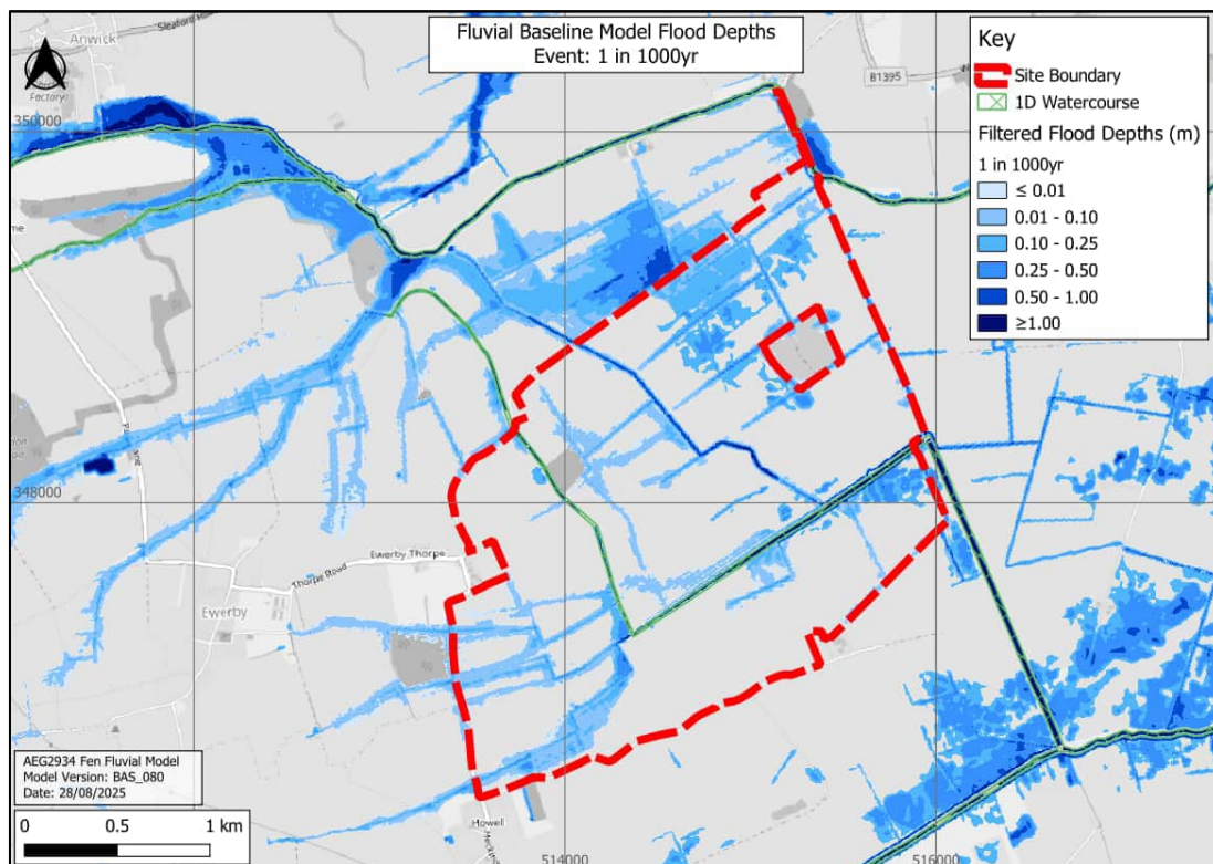
Figure 21: 1 in 1,000 year filtered modelled flood depths (Base map from OpenStreetMap and OpenStreetMap Foundation (CC-BY-SA). © nd contributors)
