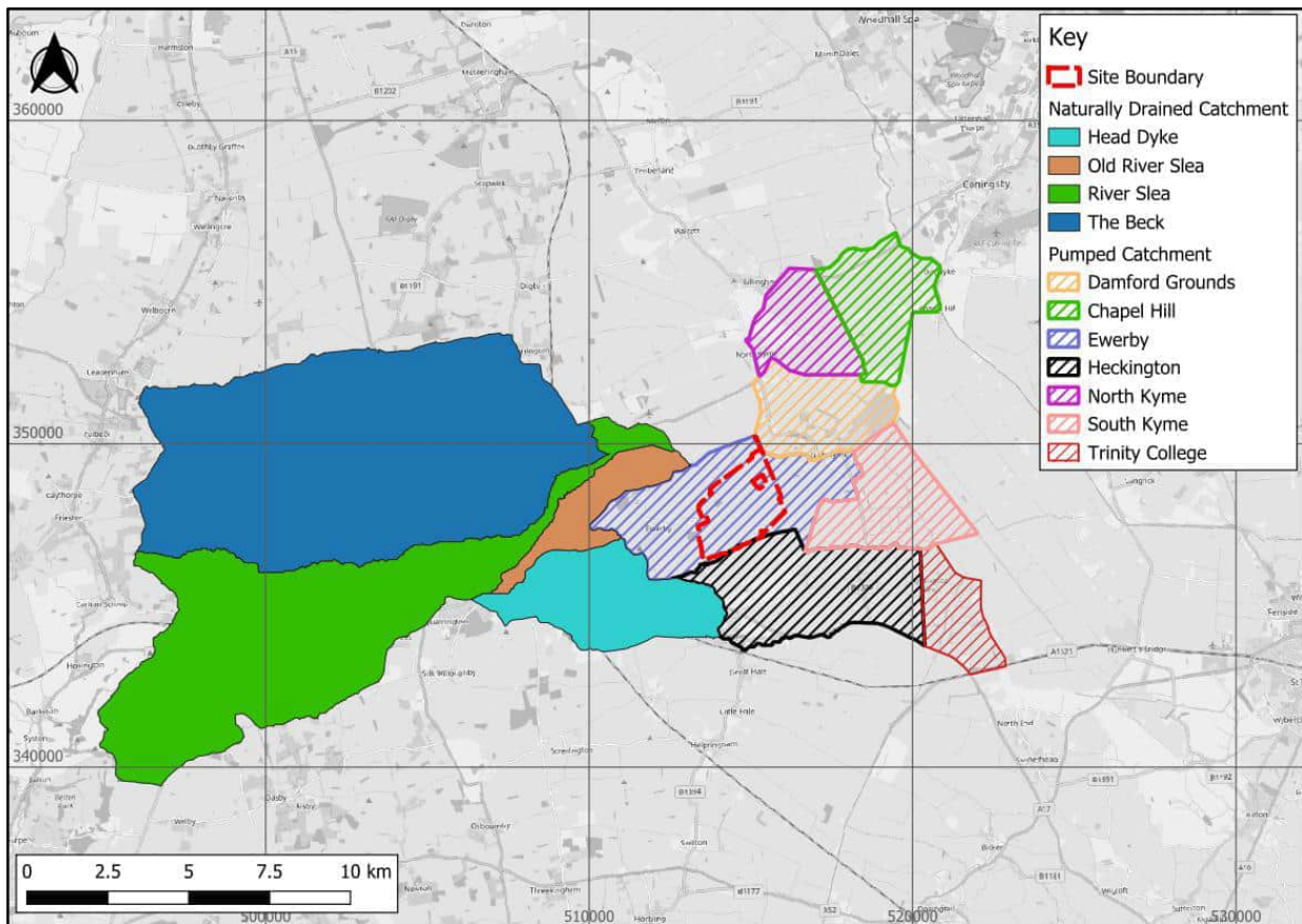
Figure 5: Natural (solid catchment) and pumped (hashed areas) catchments within the study area (Base map and data from OpenStreetMap and OpenStreetMap Foundation (CC-BY-SA). © nd contributors)
