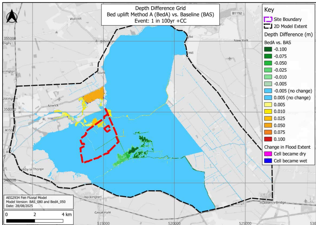
Figure 31: Depth Difference Grid - Bed uplift Method A vs. Baseline (unfiltered). Event: 1 in 100-year + CC. (Base map from OpenStreetMap and OpenStreetMap Foundation (CC-BY-SA). © [redacted] and contributors)
